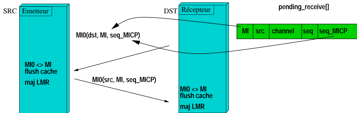
Fig. 6.7 Protocole MICP
