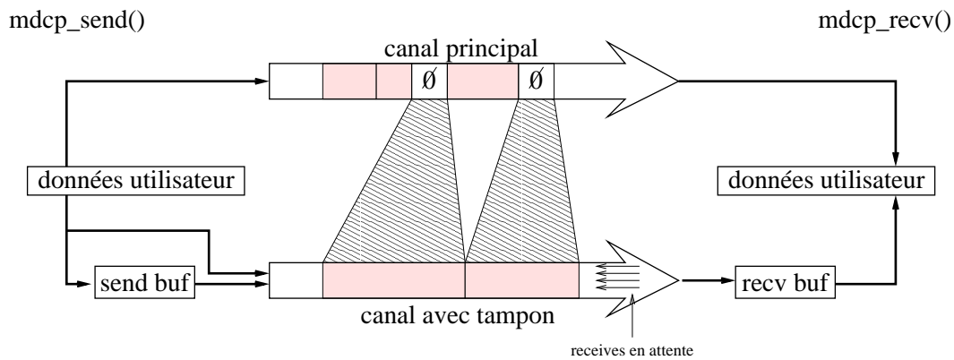
Fig. 7.6 Protocole MDCP
